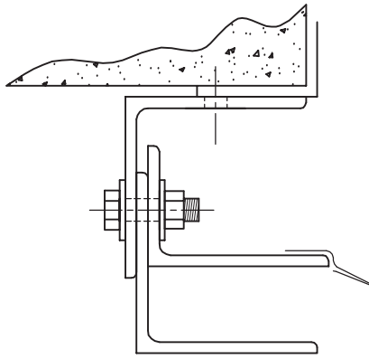
FACE OF WALL E-MOUNT TO STEEL
